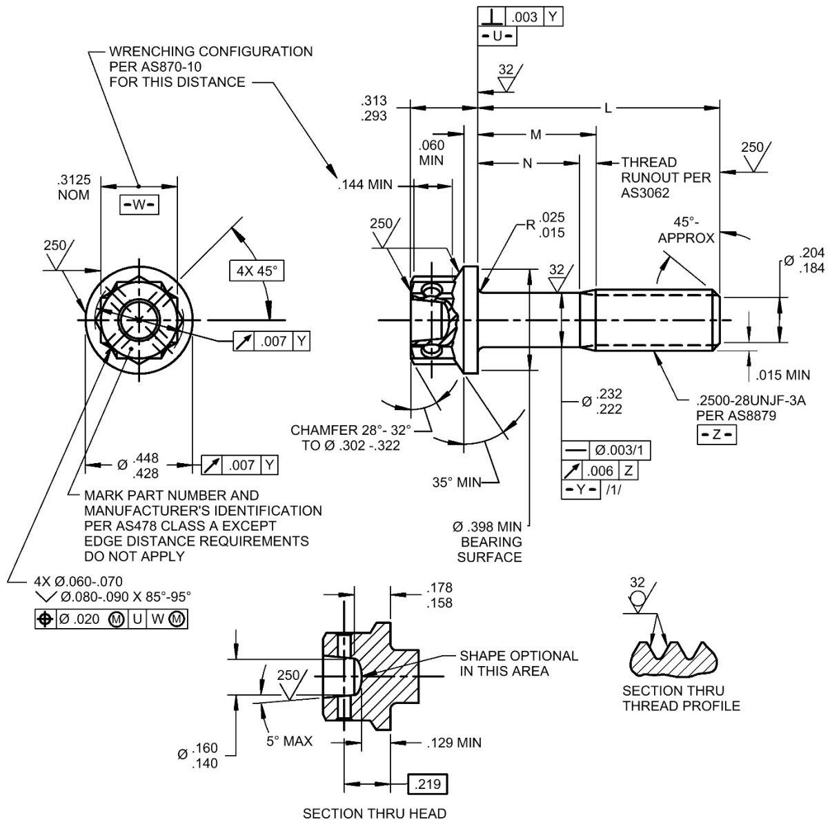
FIGURE 1 - BOLT
